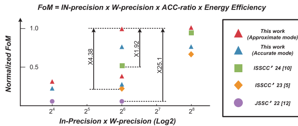
Fig. 17. Comparison of FoM with previous works.
